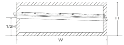
Preferred Mounting
